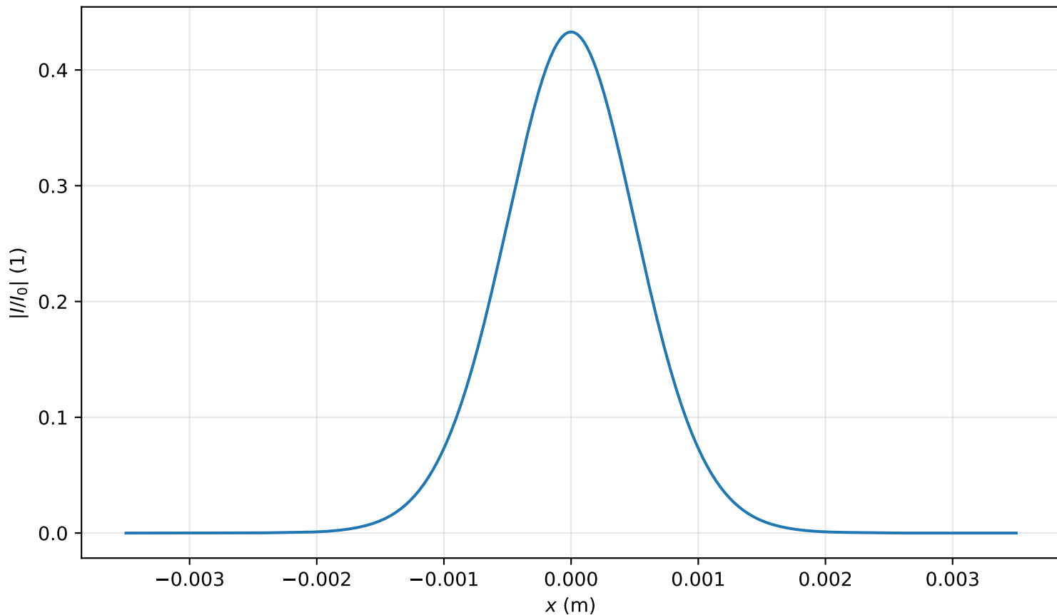
Intensity profile I(x, y = 0, z = 2.946m)/I_0 , P_{in}=0.3P_{cr} , artificial time
